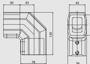
细节图 Detail drawing
