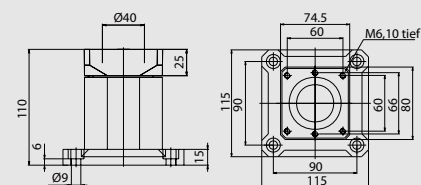
细节图 Detail drawing
