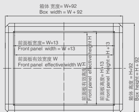
CP140 箱体尺寸 (无把手) CP140 box dimensions (without a handle)
