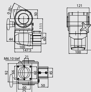
细节图 Detail drawing
