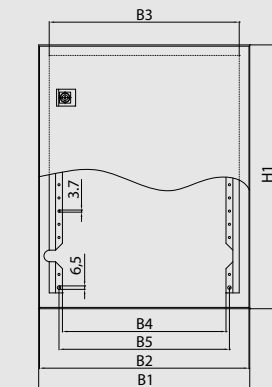
GB/BGB系列细节图 GB/BGB series detail drawing
