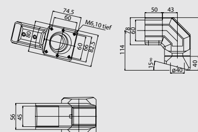
细节图 Detail drawing
