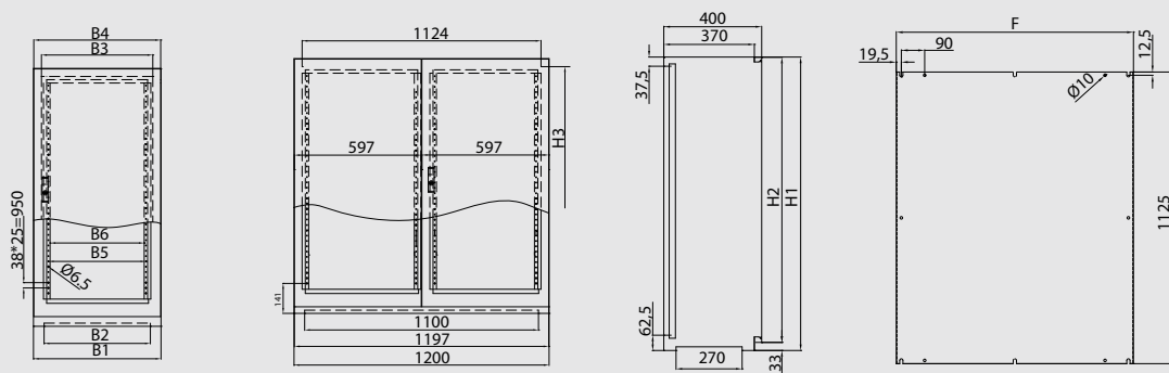
AK/BAK series detail drawing
