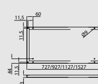
T500上部安装板 T500 upper mounting plate
