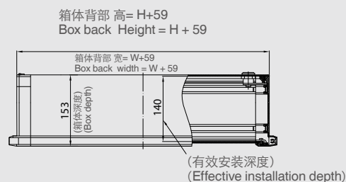
CP140 箱体尺寸 (无把手) CP140 box dimensions (without a handle)
