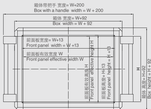
CP210 箱体尺寸 (两侧把手) CP210 Box dimensions (with handles on both sides)
