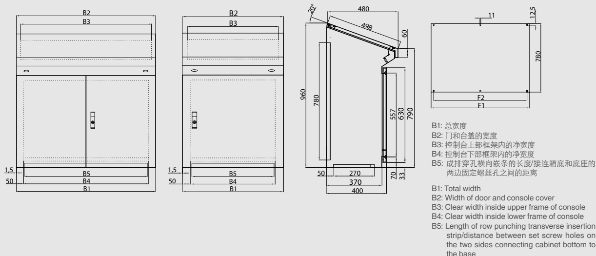
APXM series detail drawing
