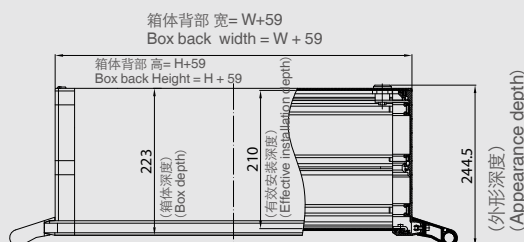
CP210 箱体尺寸 (两侧把手) CP210 Box dimensions (with handles on both sides)
