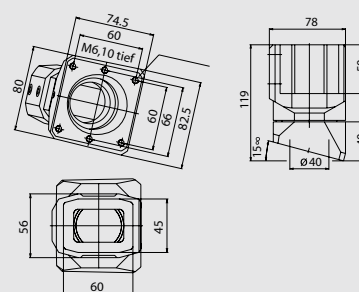
细节图 Detail drawing
