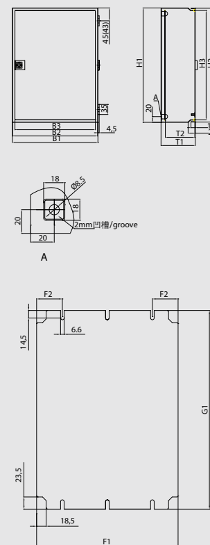
安装板细节图/Mounting Plate Detail Drawing
