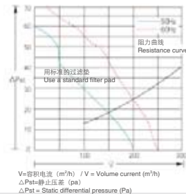
功率特性曲线 Power characteristic curve SK6621
