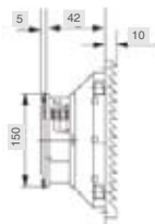
风扇及过滤器 Fan and filter SK6621. 230
