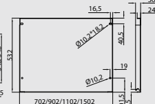
T500下部安装板 T500 lower mounting plate
