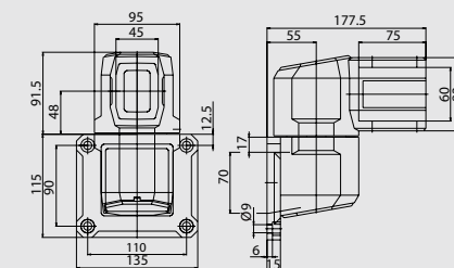
细节图 Detail drawing
