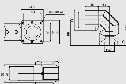
细节图Detail drawing
