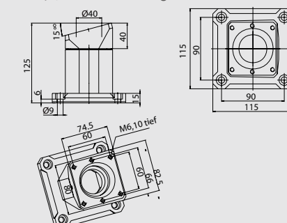
细节图 Detail drawing
