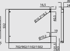
T500下部安装板 T500 lower mounting plate
