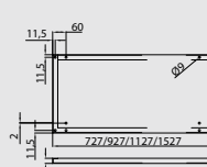
T500上部安装板 T500 upper mounting plate
