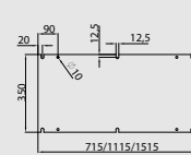
T400上部安装板 T400 upper mounting plate
