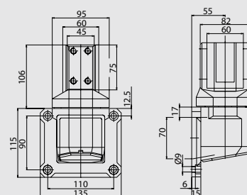
细节图 Detail drawing
